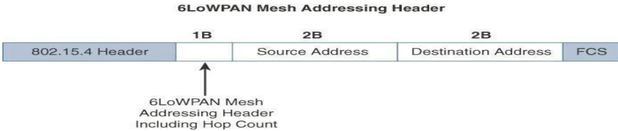
Figure 3.6 6LoWPAN Mesh Addressing Header
