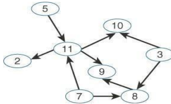
Figure 3.8 Example of a Directed Acyclic Graph (DAG)
