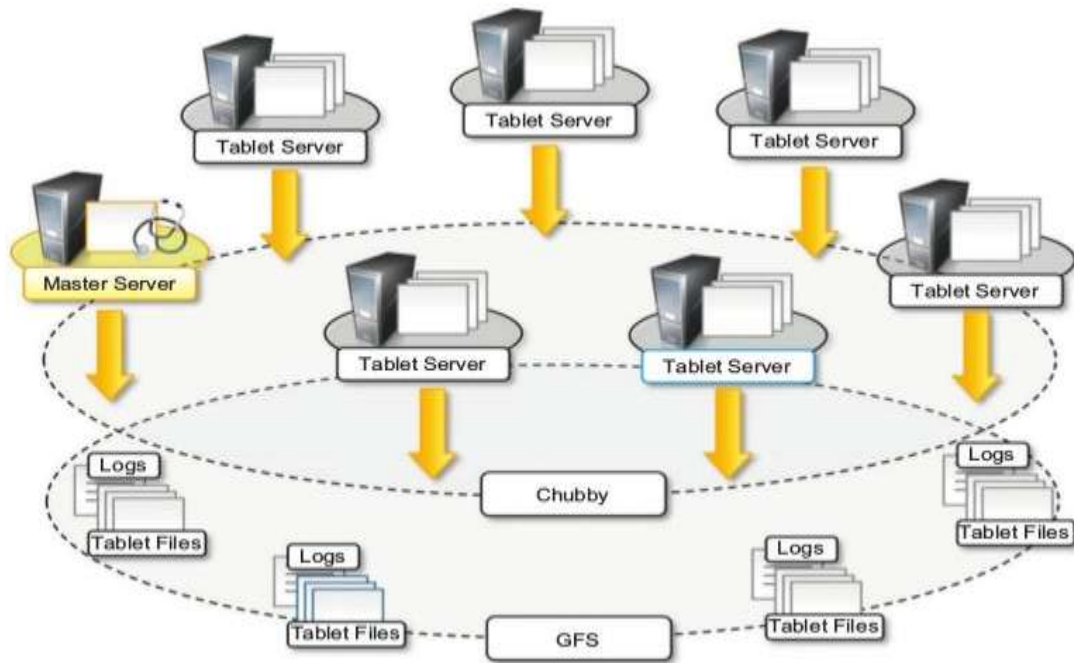
FIGURE 8.4 Bigtable architecture.
